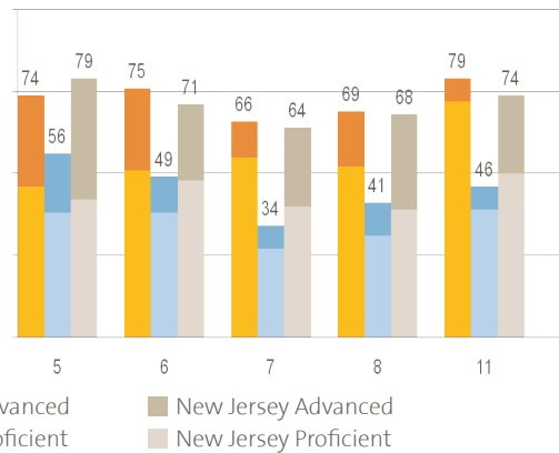
MATHEMATICS
